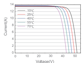
Current-Voltage Curve JAM72D30-540/MB/1500V
